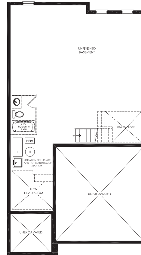
BASEMENT PLAN ELEV. 'A', 'B' & 'D'
