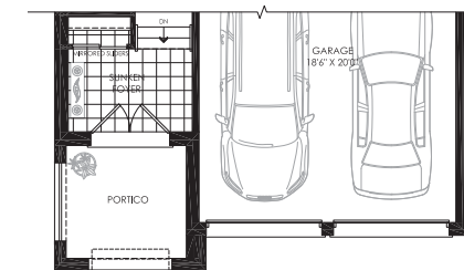
PARTIAL GROUND FLOOR PLAN ELEV. 'D'
