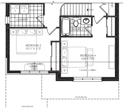
PARTIAL SECOND FLOOR FLEX PLAN ELEV. 'B' 4 BEDROOM LAYOUT
