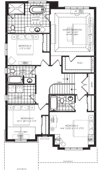
SECOND FLOOR FLEX PLAN ELEV. 'A' 4 BEDROOM LAYOUT
