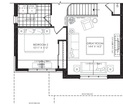
PARTIAL SECOND FLOOR PLAN ELEV. 'B'
